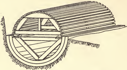
FIG. 25.—CENTRE FOR BRICK SEWERS.
